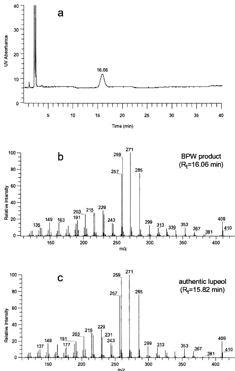
Fig. 2. LC-APCI-MS Analysis of the Product by pOSC BPW
