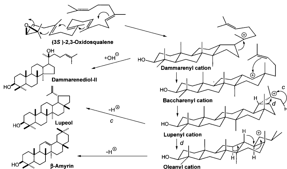
Fig. 6. Cyclization of Oxidosqualene to Dammarenediol-II, Lupeol and \beta -Amyrin
